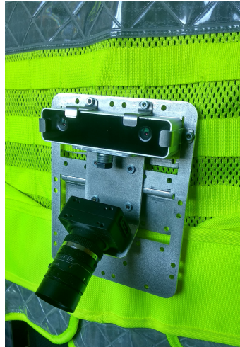
Figure 2.6: Safety Vest with the sensor setup that consists of an IMU-aided stereo camera and a downward-looking monocular camera. This placement of the sensors was chosen since it will not disturb the human when performing the usual tasks. Furthermore, cameras cannot get obstructed by hands, and this part of the human body is the most stable and has the smallest chance of doing abrupt motion that could blur the images.
