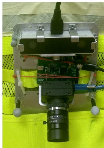
Figure 2.12: The visual sensor suite, stereo and monocular camera, upgraded with the UWB sensor.
