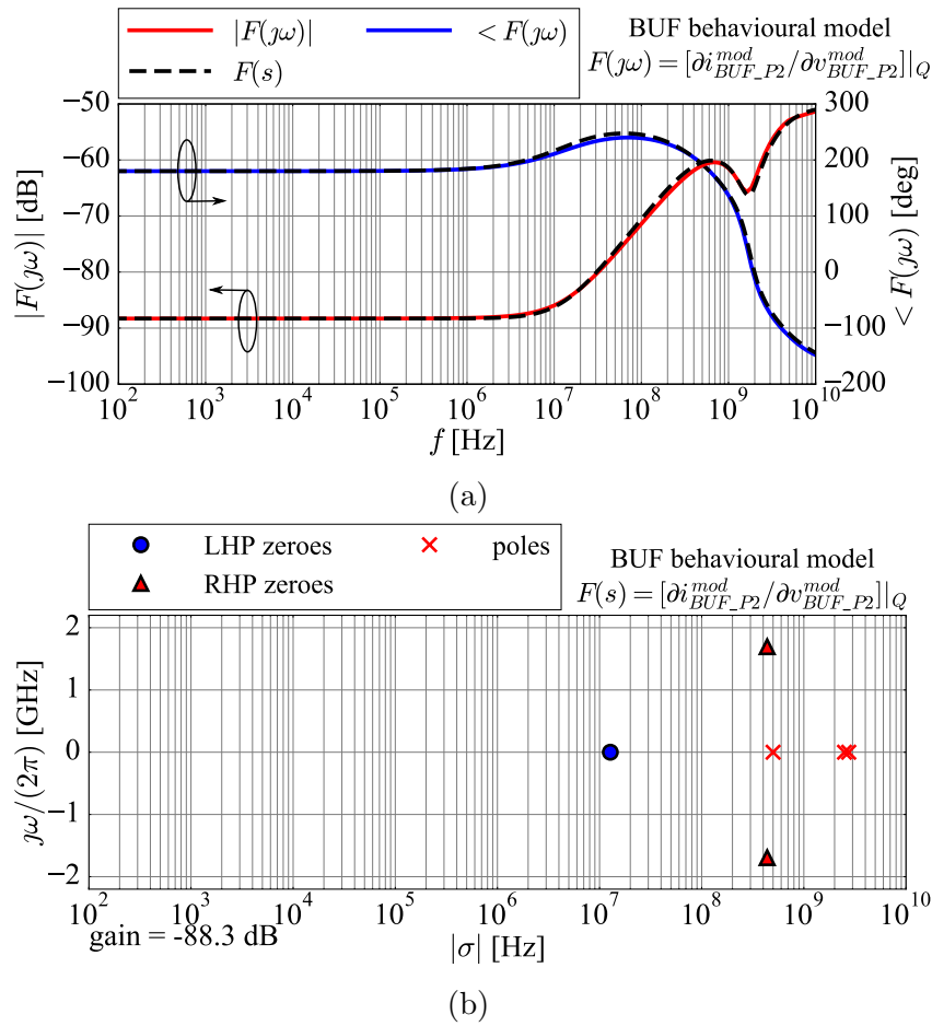
Figure 3.18: (a) Frequency response BUF_{mod_{22}}(j\omega) of the transfer function from the input voltage v_{BUF\_P2} to the input current i_{BUF\_P2} of the BUF behavioural model, obtained by simulations (solid lines), and the frequency response of the fitted transfer function with the poles and zeroes shown in (b) (dashed lines), (b) positions of the 3 poles and 1 zero in the LHP, and the 2 zeroes in the RHP of the s -domain of the analytical small-signal mode BUF_{mod_{22}}(s) [38].
