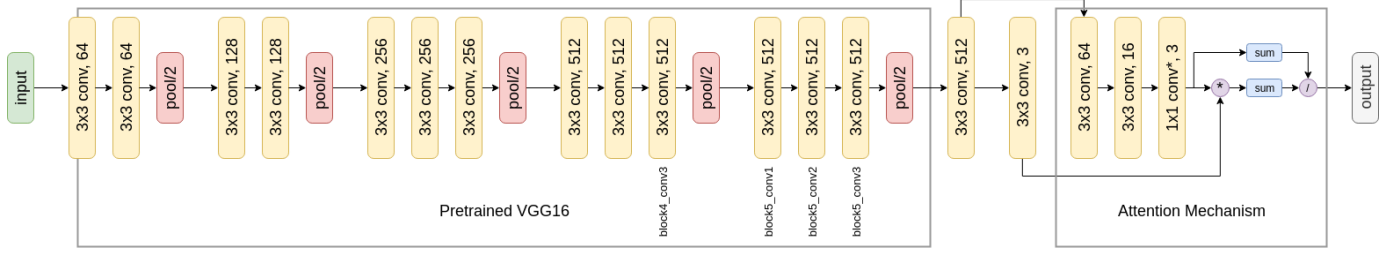
Fig. 2: Illustration of the proposed architecture with the attention mechanism. The conv* operation uses a different set of weights for each patch of the input, i.e. the weights are unshared. Operators '*' and '/' resemble the element-wise multiplication and division of two feature maps, respectively. Sum is a simple sum pooling operation.
