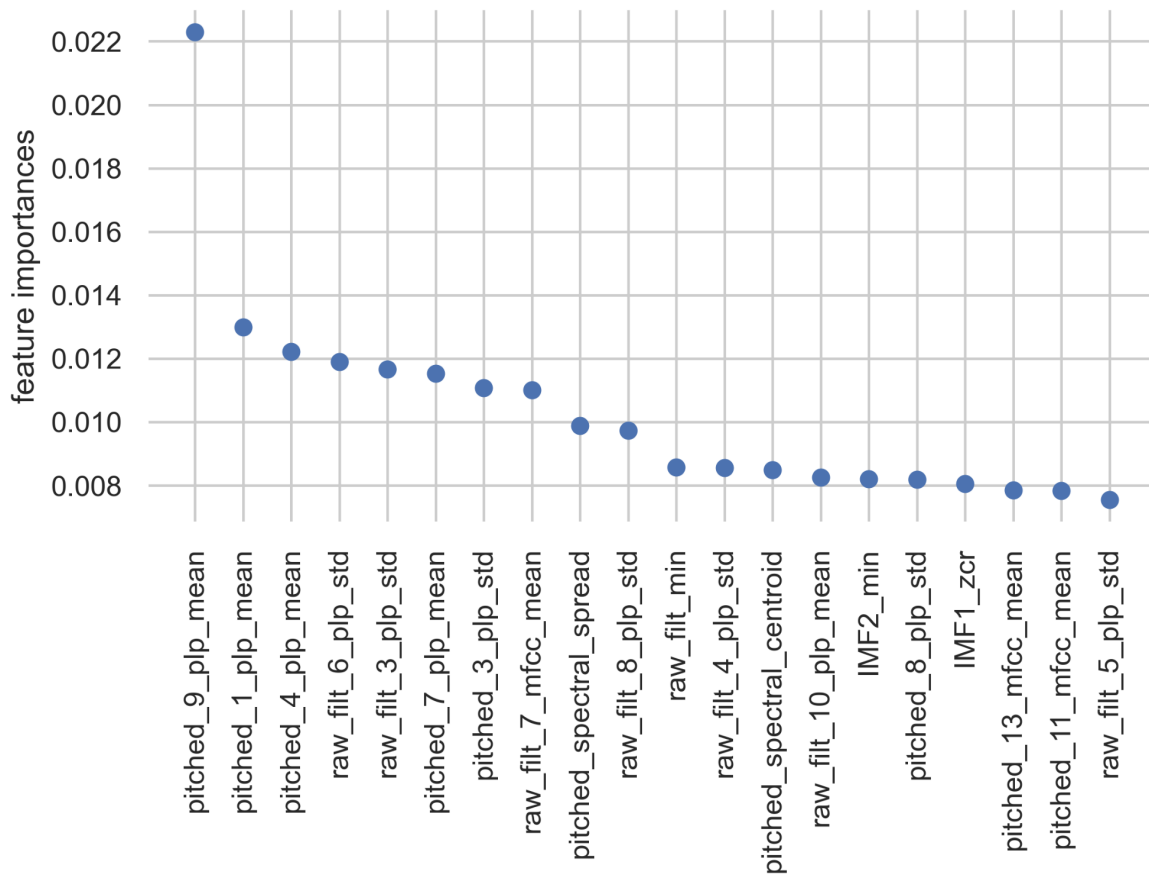
Figure 4.21. The top 20 features inherently obtained by the learning algorithm of the support vector machine classifier. Custom dataset with 150 ms window used as an input.
