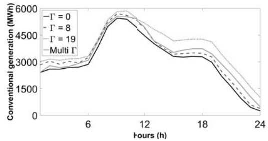
Fig. 1. Conventional generation.
