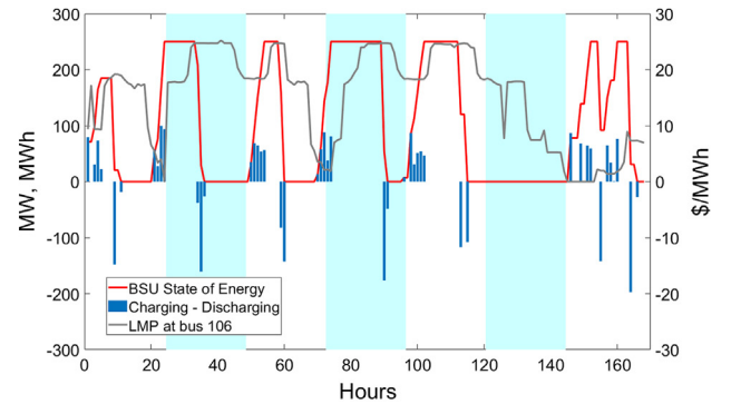
(a) BSU at bus 106
