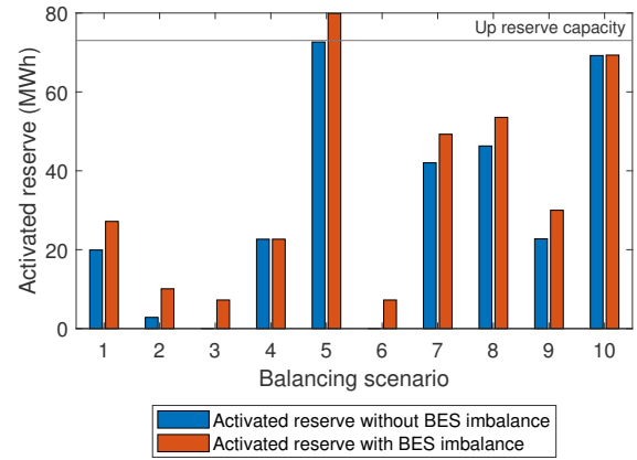
Fig. 7. Sum of the generators' deployed up reserve capacity per balancing scenario in hour 21 with and without imbalance caused by the BES.
