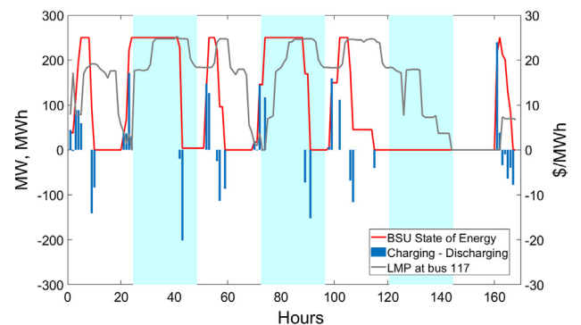
(b) BSU at bus 117
