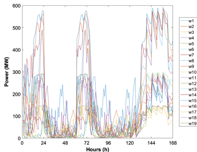
Fig. 2. Available output of 19 wind farms within the IEEE-RTS 96 during the representative week [54].
