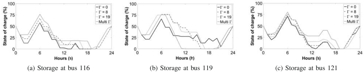
Fig. 2. Storage operation.
