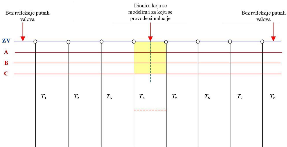
Slika 7.4: Model dalekovoda [103]
