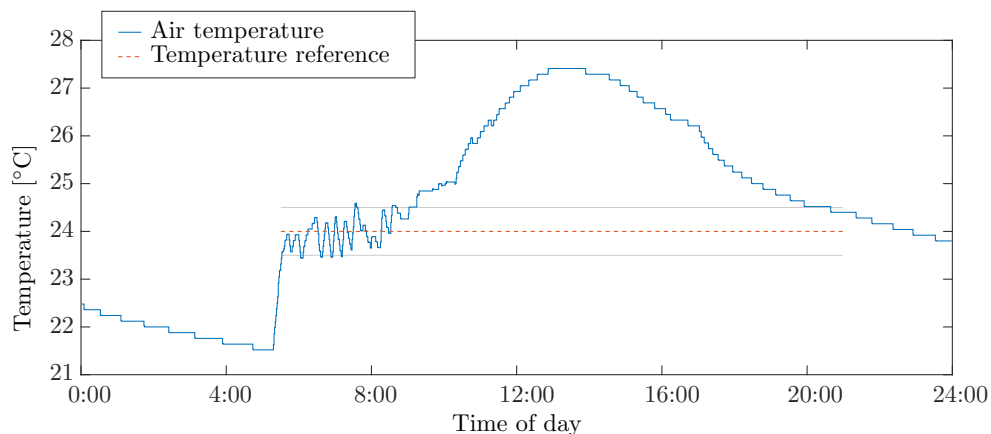
Figure 8.23. Zone temperature in one exemplary south-oriented zone on 15 January 2020.
