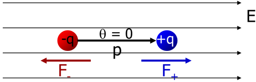
Figure-2.3: Mechanism of molecular polarization in electric field
