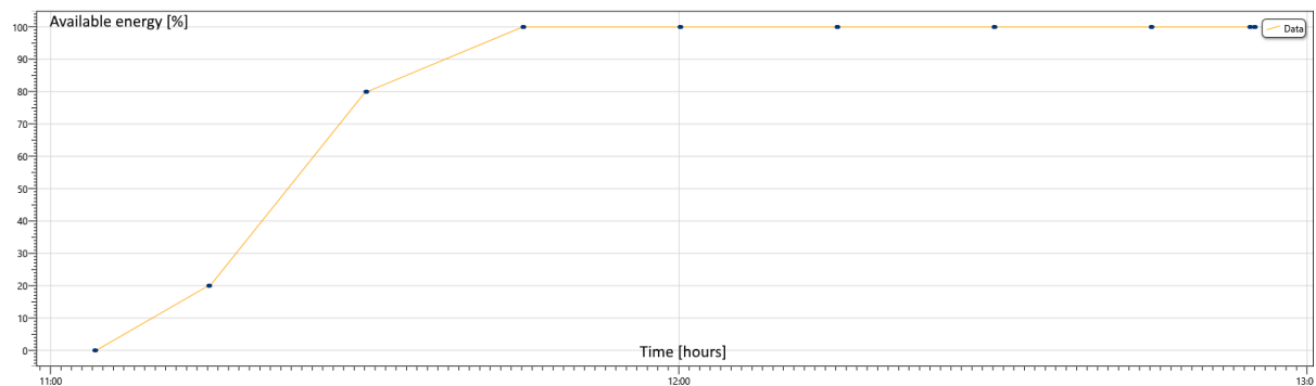
Figure 5.2. Supercapacitor charged by solar energy. 80% of the available energy (3.38 V) is reached within 40 minutes after the test start. Initial voltage at the supercapacitor was 2.2 V.
