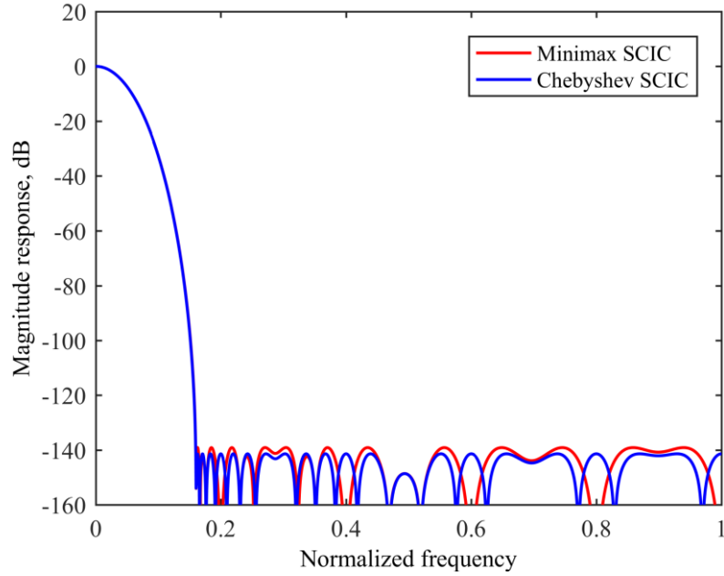
Figure 4.8 Magnitude responses of sharpened CIC filter with N = 2 and R = 10 , obtained by minimax SPT sharpening with M = 4 and P = 2 , and by Chebyshev sharpening of fourth-order [61], assuming \omega_p = 0.4\pi [76].
