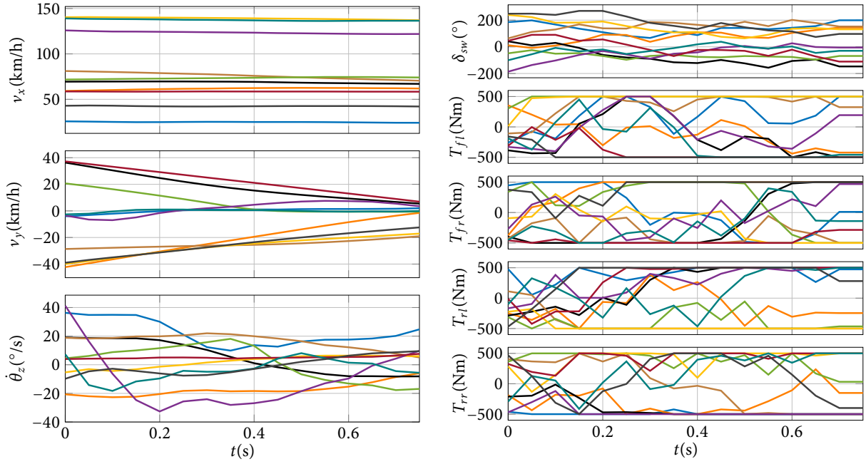
Figure 5.3: Example state (on the left) and input (on the right) trajectories.
