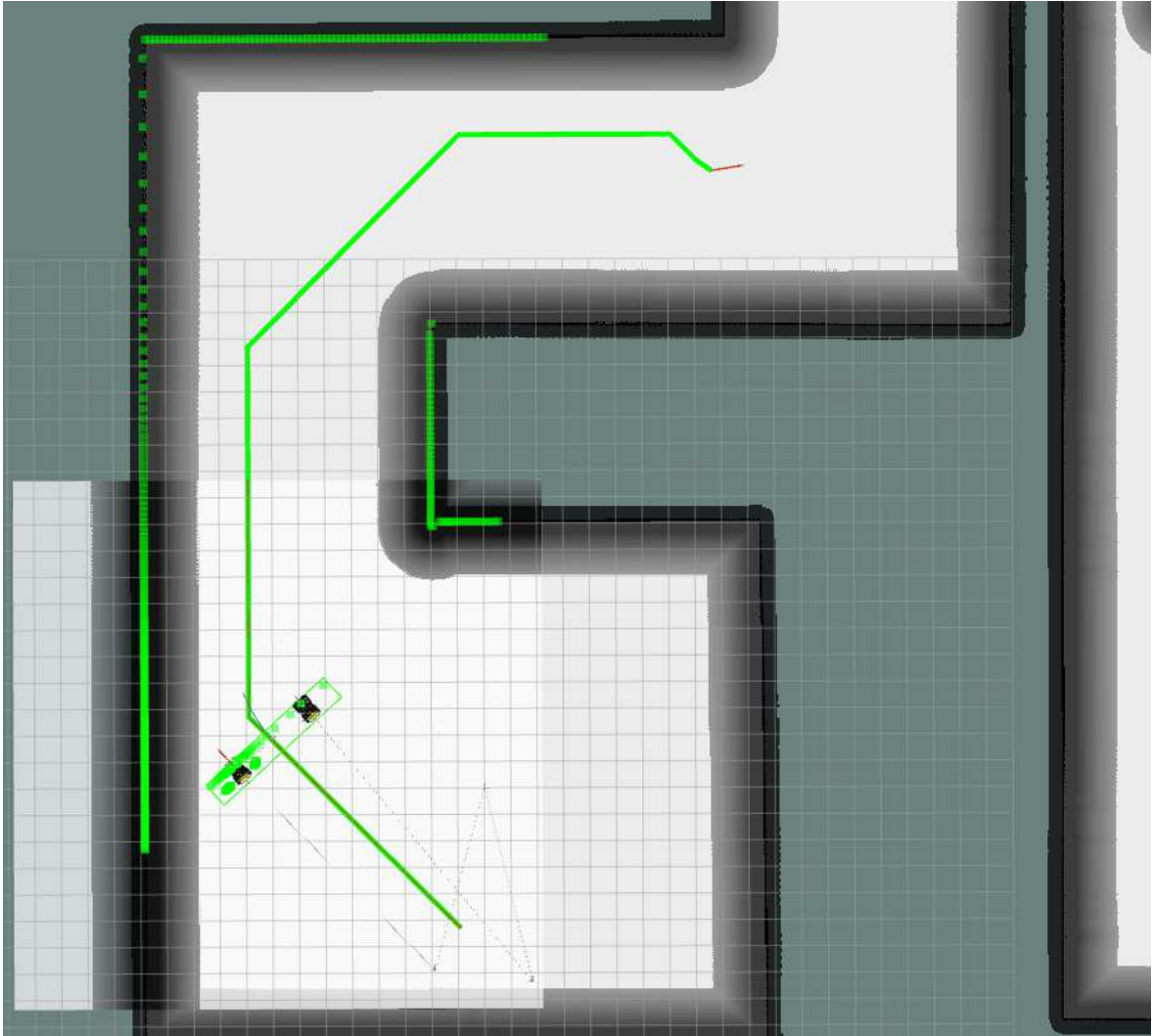
Figure 5.3: RViz simulation
