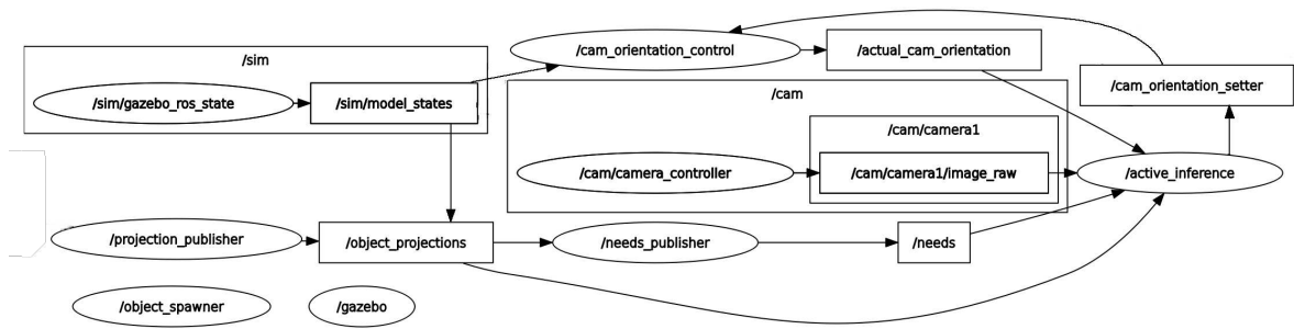
Figure 4.2: Node graph during simulation
