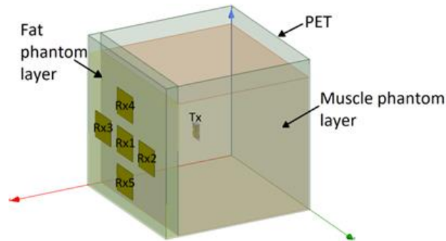
Figure 3.6: Simulated phantom container [65]
