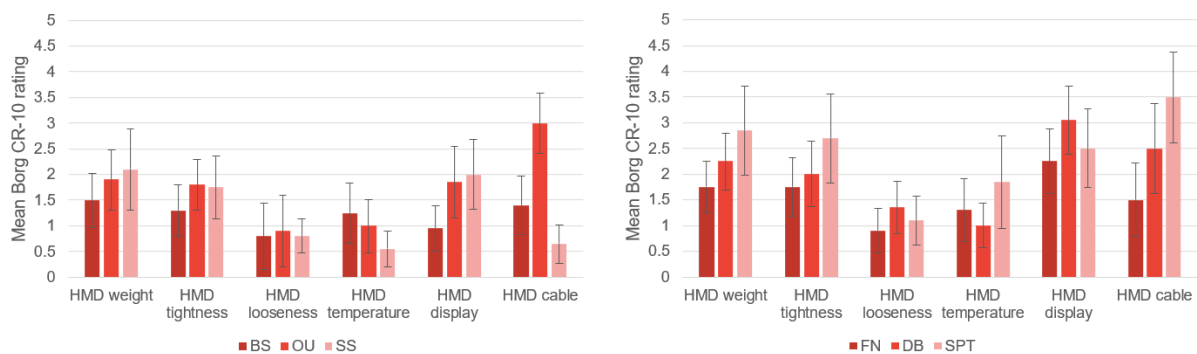
Figure 5.4: Mean Borg CR-10 ratings (95% CI) for discomfort and annoyance related to different device factors ( Study 1 – left, Study 2 – right; taken from [30])
