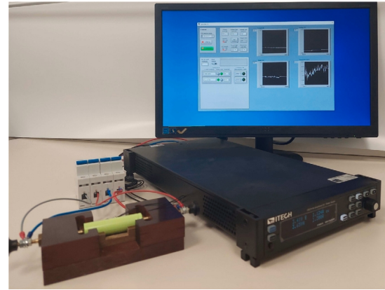
Fig. 2. Experimental setup.
