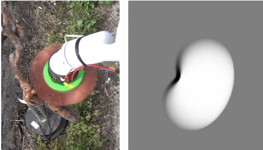
Figure 4.15: Occupancy grid mapping at a constant tool height during the suckering experiment. The map is built online, being constantly updated during the experiment.
