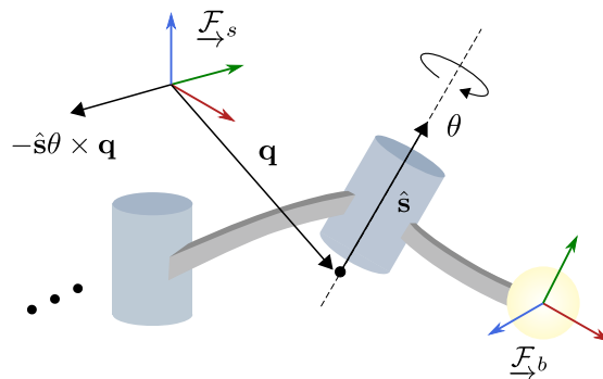
Figure 3.2: Sketch of the parameterization of link motions for revolute joints using screws. The vector \hat{\mathbf{s}} is the joint's rotation axis, while \mathbf{q} is the position of some point on the rotation axis in the robot's home configuration (i.e., \theta = 0 ).
