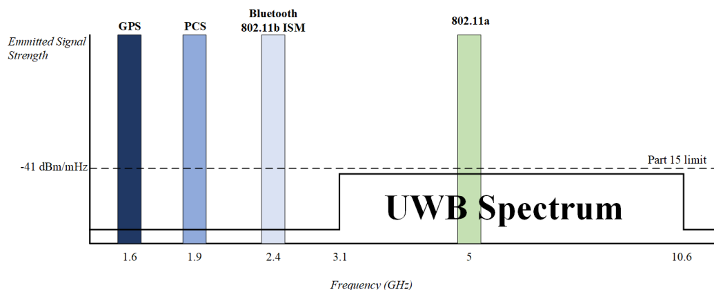
Figure 3.2 UWB spectrum and the FCC requirements
