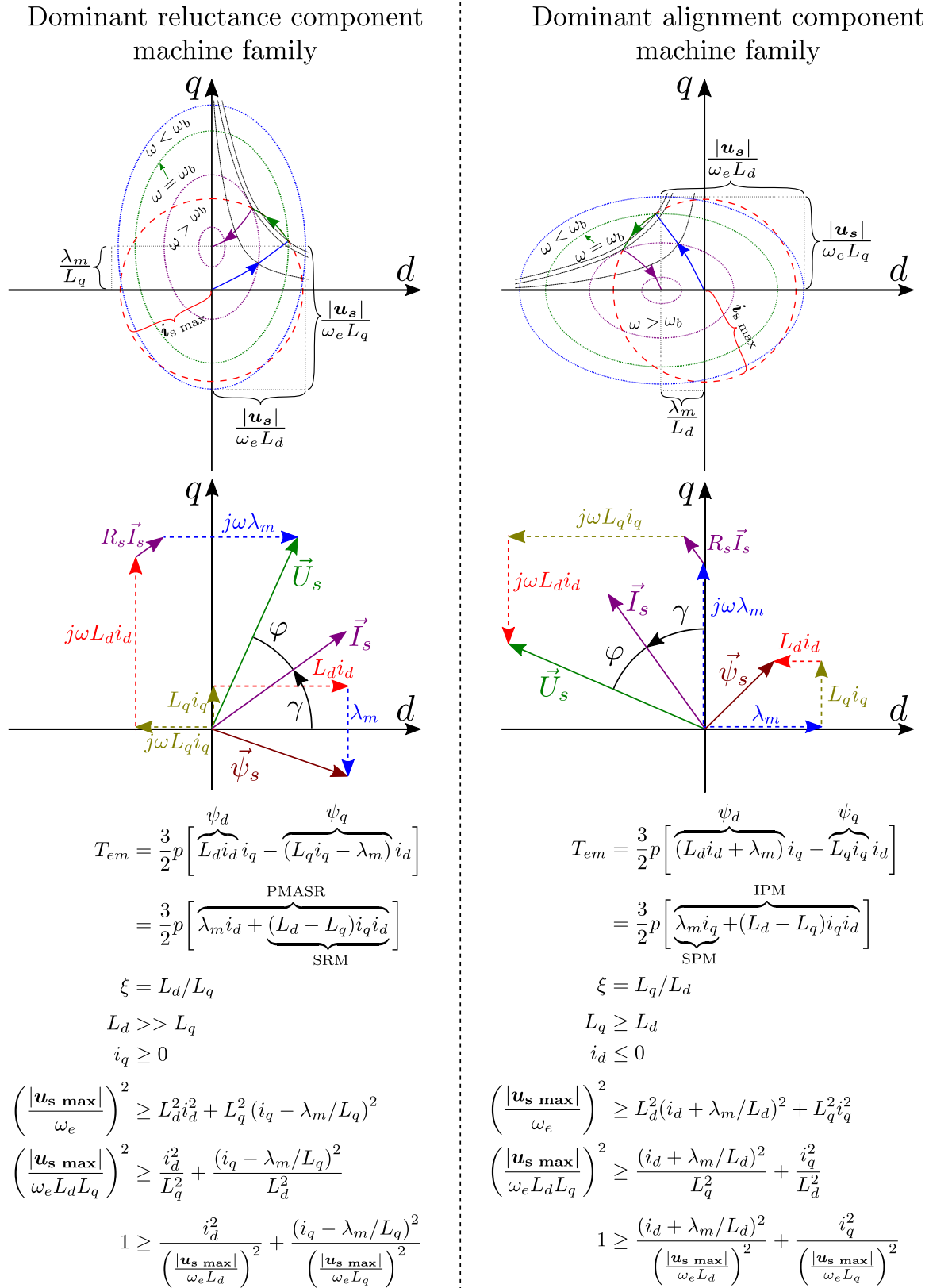
Fig. 17: Voltage and current constrains, voltage vector diagrams and equations for dominant reluctance torque component family (left) and dominant alignment torque component family (right).
