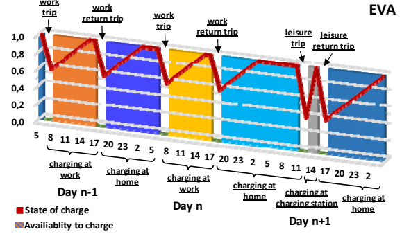
Figure 2. EV's driving/parking/charging behavior under conventional EVA
