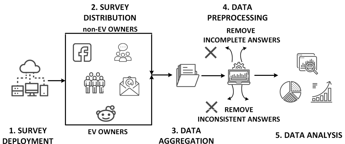
Figure 3.1: Research methodology
