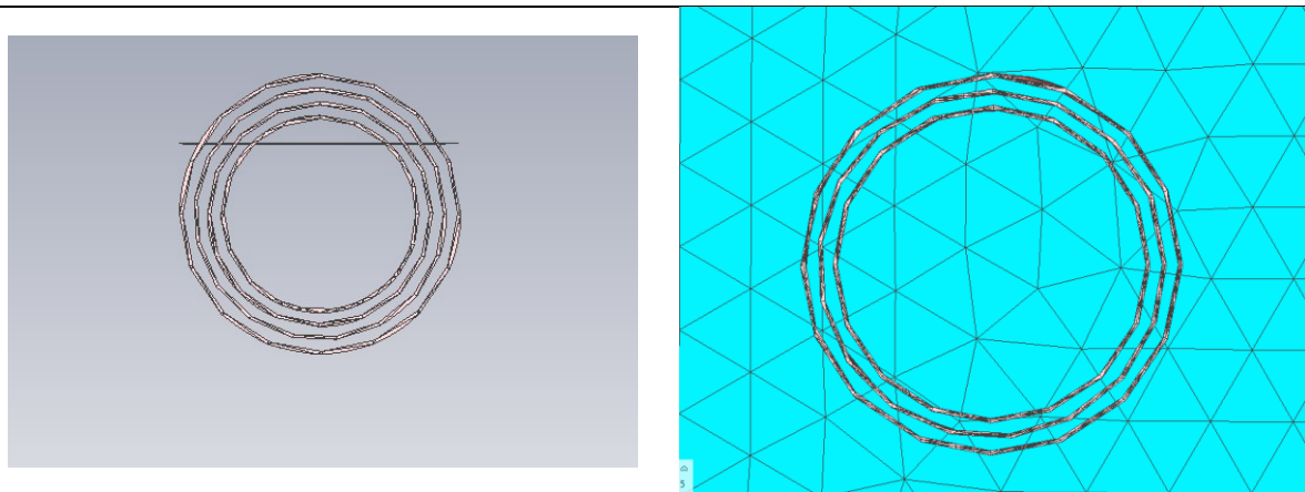
Figure 19. FEM model of transmitter coil (left) and receiver coil (right).
