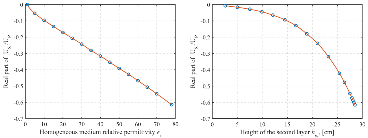
Figure 63. Real part of FEM sensor response data for the homogeneous case (left) and double-layered case (right) at 25 MHz. Blue circles are FEM data, and the red line is interpolated data.
