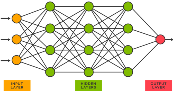
Figure 35. Neural network
