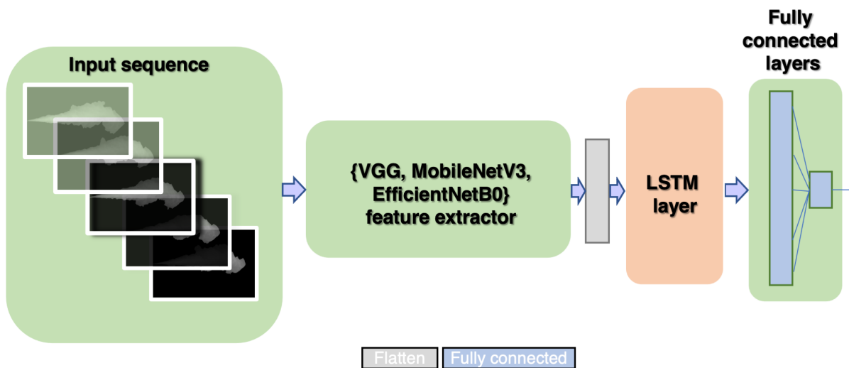
Figure 5.8: CNN-LSTM architecture
