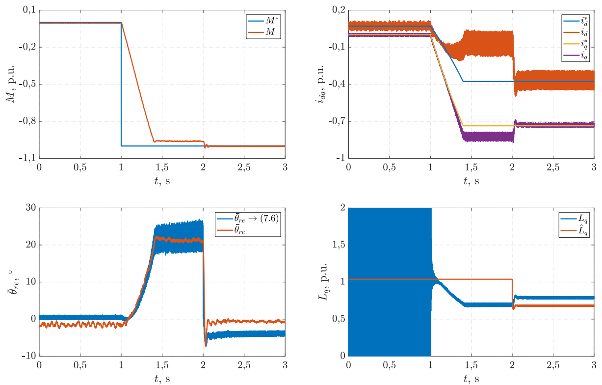
(a) PMSG1
