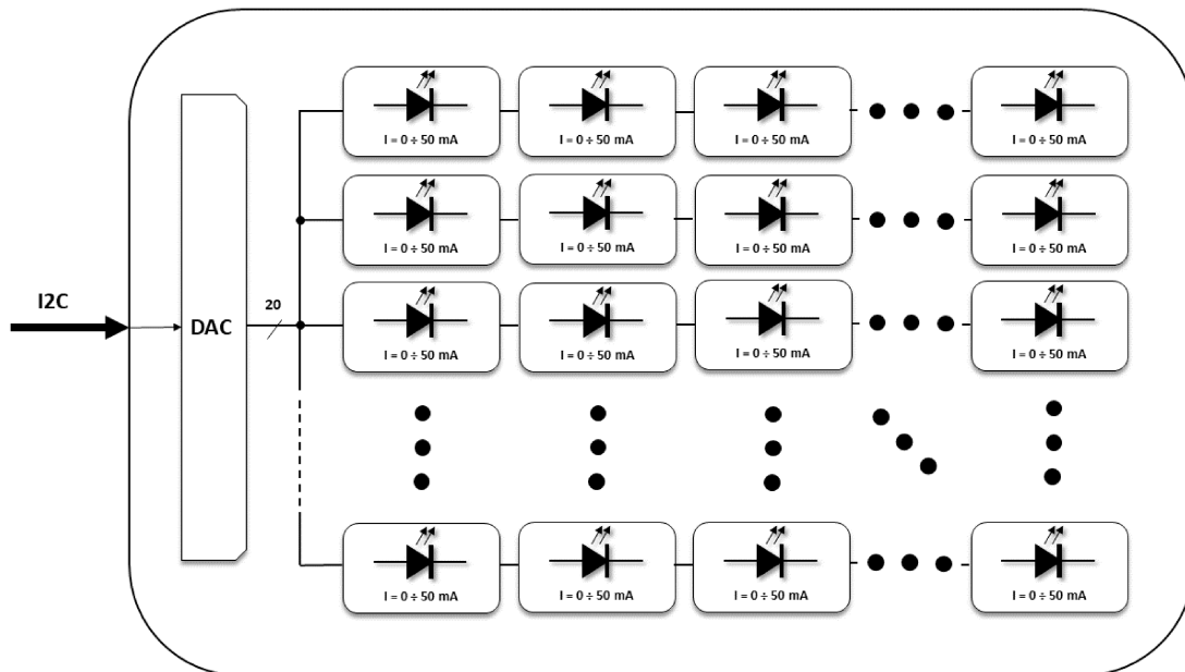
Figure 3 - Light-source array
