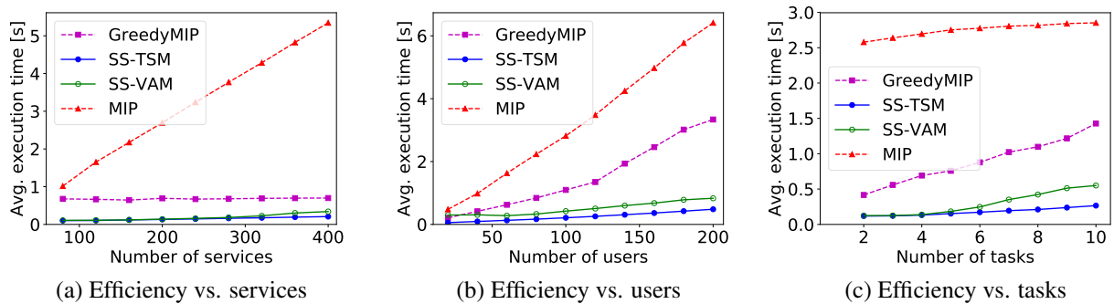
Figure 6.23: General Experiment: time vs. number of services/user/tasks
