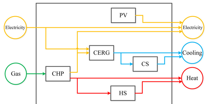
Fig. 1. Energy hub.
