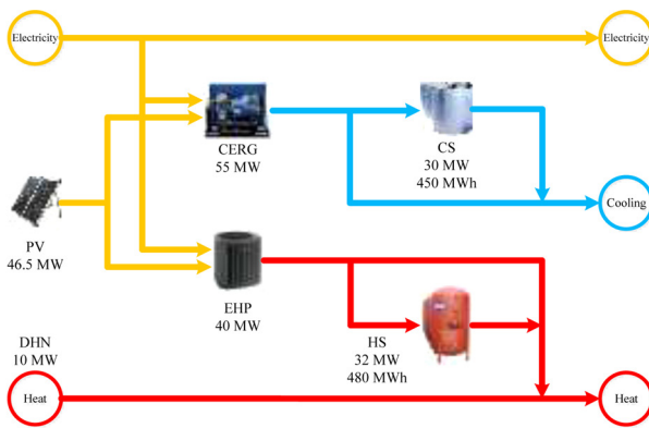
(a) Alternative planning scheme 1 (Focus: PV+HS/CS)
