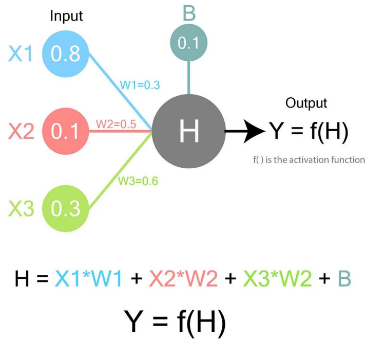
Figure 3.1: Single neuron functionality [10]
