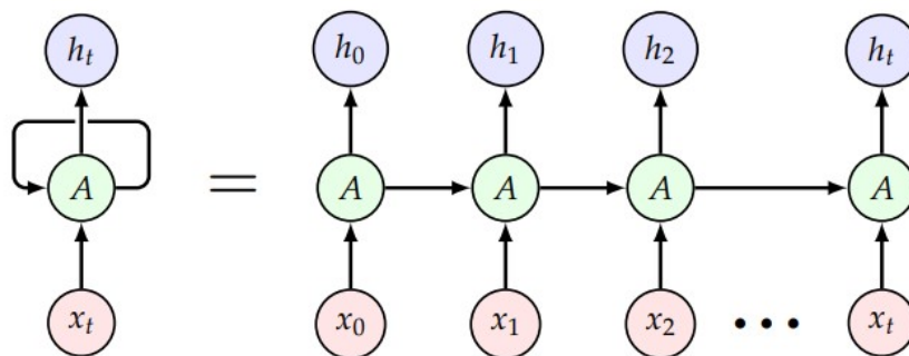
Figure 3.4: Unrolled RNN structure [16]
