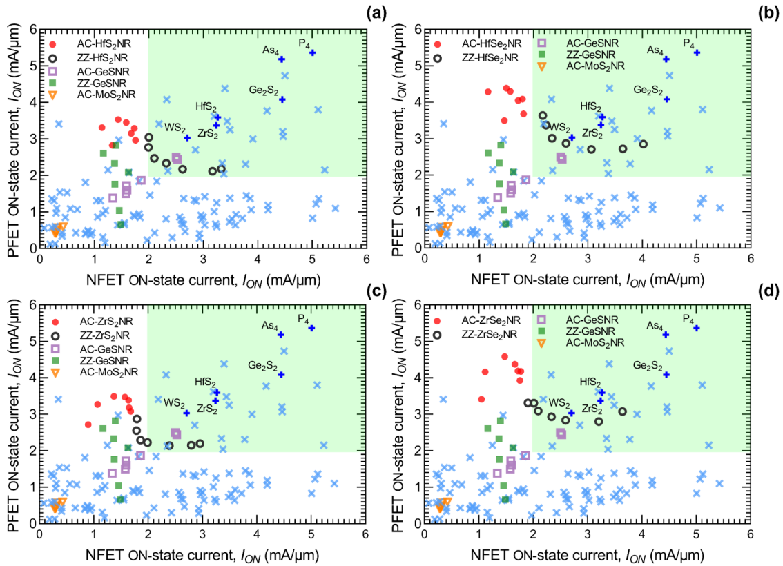
FIG. 9. nFET vs pFET ON-state current of devices with (a) AC and ZZ-HfS 2 NR, (b) AC and ZZ-HfSe 2 NR, (c) AC and ZZ-ZrS 2 NR, and (d) AC and ZZ-ZrSe 2 NR channel. Green area represents IRDS I_{ON} requirement with I_{ON} = 1.979 \text{ mA}/\mu\text{m} . The 100 2DMs reported in Ref. 12 are included in graphs with the most relevant materials directly named and marked with blue plus signs, while the unnamed 2DMs are shown with light blue crosses.
