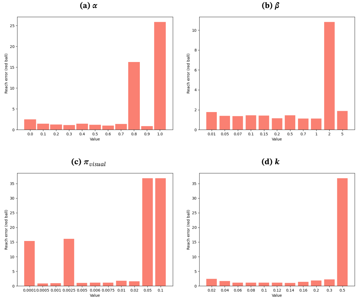
Figure B.2: Reach error for different values of \alpha , \beta , \pi_{visual} and k
