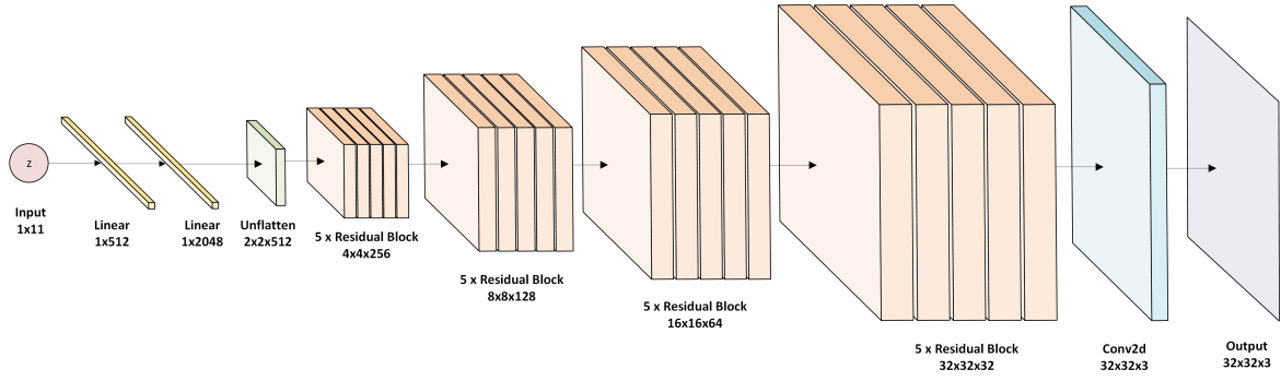
Figure 4.5: Decoder architecture
