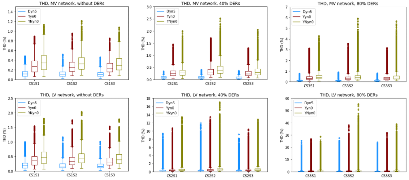
Fig. 3. THD(%) - results
