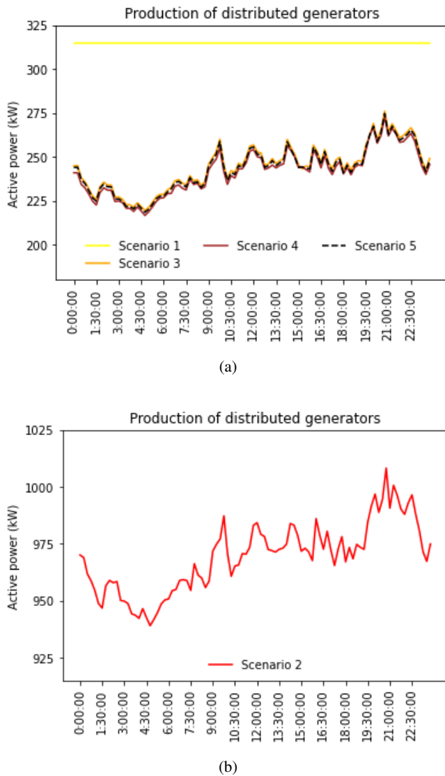
Fig. 4: Calculated export DOEs - Case Study 2b
