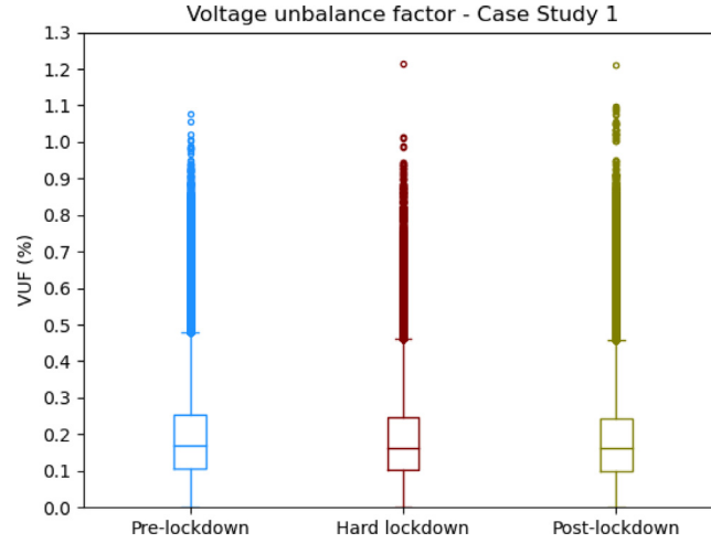
Fig. 4. Voltage unbalance facotr (%) - CS1.
