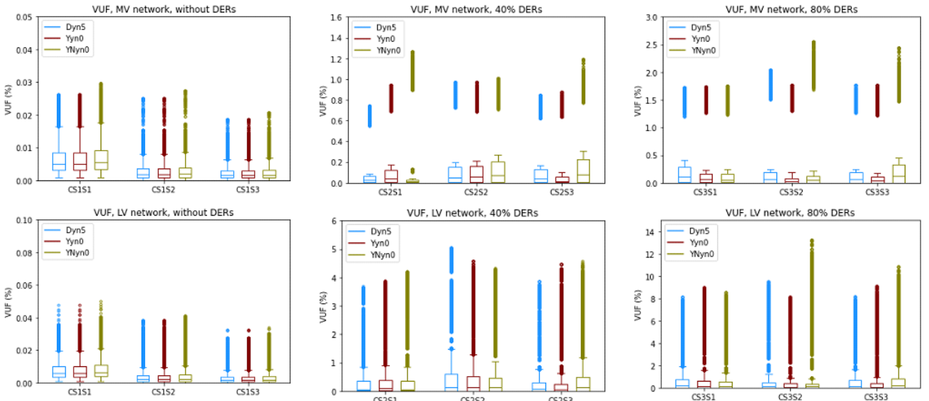
Fig. 2. VUF(%) - results
